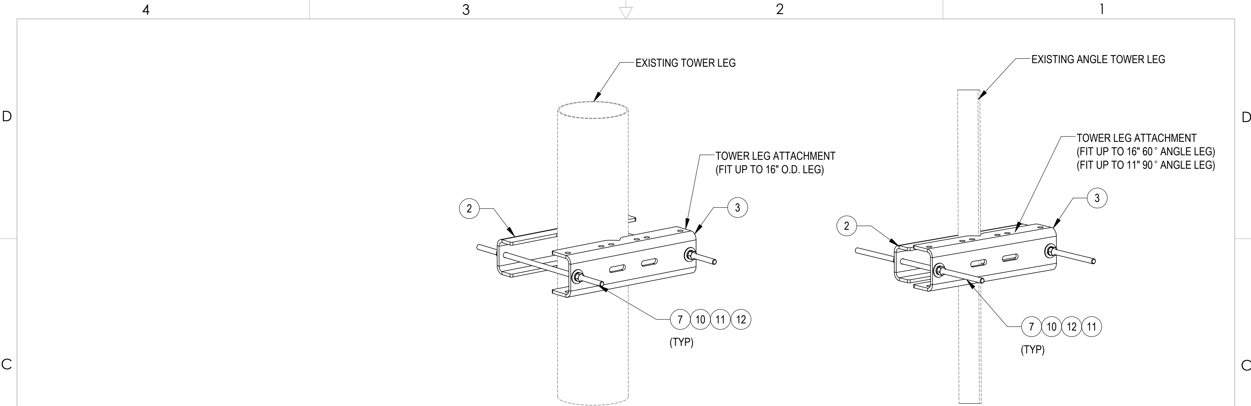
ROUND TOWER LEG ATTACHMENT DETAIL
