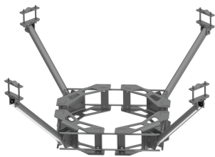
Monopole Load Distribution Reinforcement Kit, 4 Sector, 10" to 30" OD, 60" Kicker
