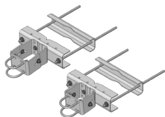
Large Leg Universal Open Face Pipe Mount Kit for 4-1/2 in OD pipe
