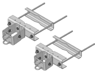
Large Leg Universal Open Face Pipe Mount Kit for 2-3/8 in OD pipe
