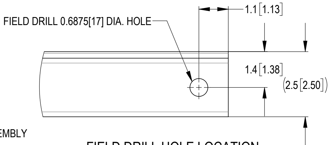
FIELD DRILL HOLE LOCATION DETAIL "A"
