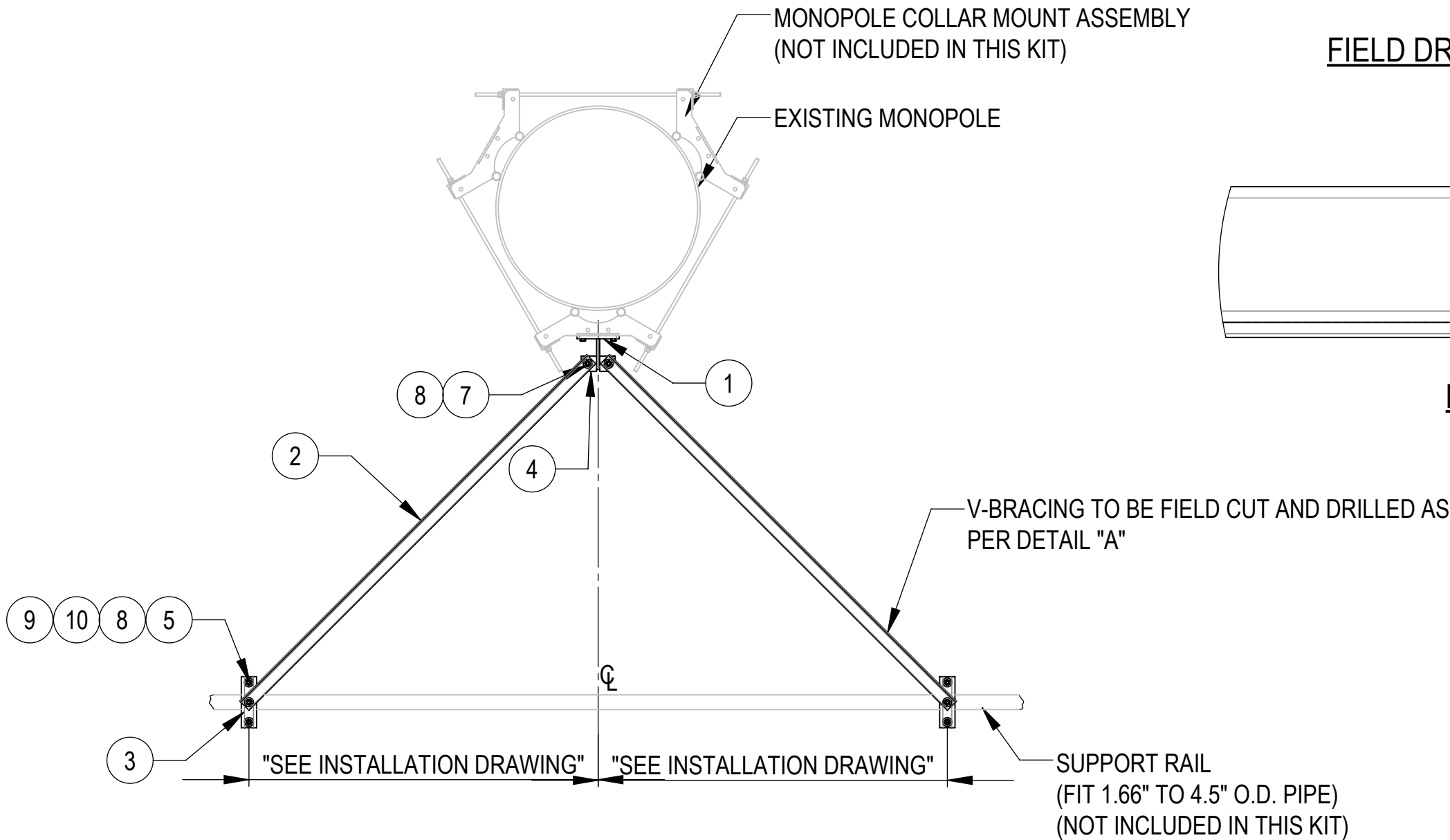
V-BRACING KIT FOR MONOPOLE
