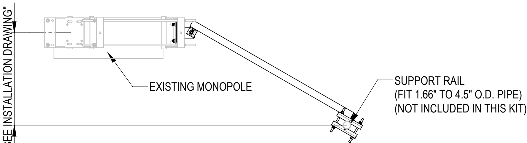
V-BRACING KIT - VERTICAL (OPTION-2)
