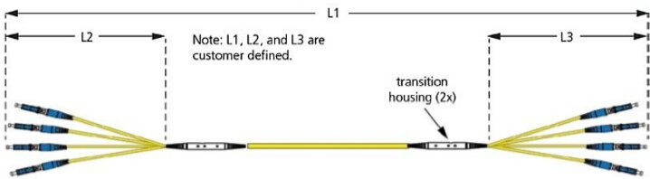
24 – 144 Fiber Assembly Image
