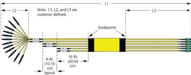
MPO Connectors on Side B (Optional)
