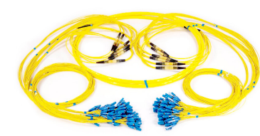
Fiber Optic Patch Cord, Multi-fiber, Singlemode, SC/APC to LC/APC, Yellow
