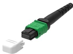
Fiber Optic Connector Kit, multimode, OM3/OM4, MPO-16/APC, ULL, non-pinned, green, for 3 mm cable
