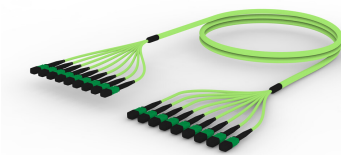
Ultra Low Loss (ULL) OM5 MPO16 (Pinned) to MPO16 (Pinned), Fiber Trunk Cable Assembly, 144-Fiber, Dual Rated (OFNR/LSZH)
