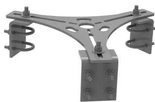
Small Cell Antenna Pole Top Mount (for use with SCSMRU-301-T Small Cell Ring Mount)
