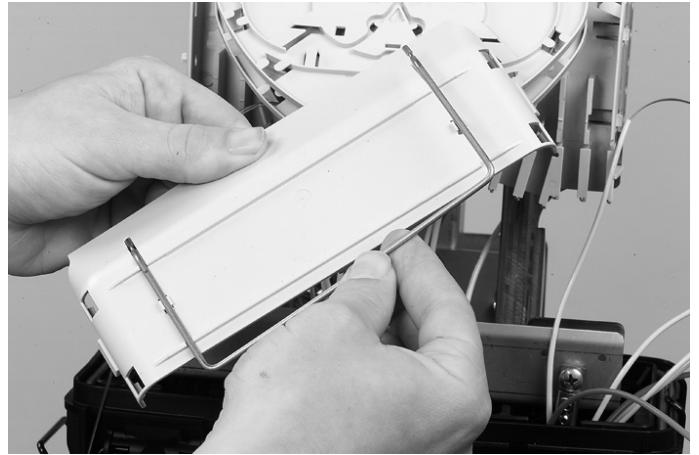
9.1.1.1. Remove the strap and the routing block cap. To remove the routing block cap, lift the two snaps on one side of the routing block cap.
