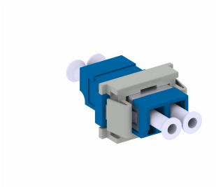
Fiber Optic Duplex Adapter, Singlemode LC/UPC, blue, with FIST retainer
