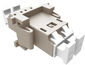
Fiber Optic Duplex Adapter, Multimode LC/UPC, beige, with FIST retainer
