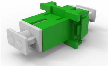
Fiber Optic Simplex Adapter, Singlemode SC/APC, green, with FIST retainer, 24 pcs
