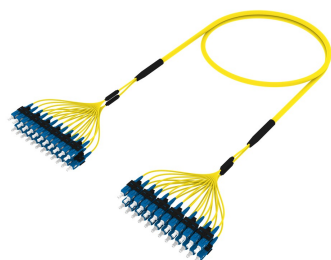
Fiber Optic Patch Cord, OS2, SC/UPC-SC/UPC, 24F RBR, 2.0 mm subunits, 84 m, yellow, 39"/60" breakouts
