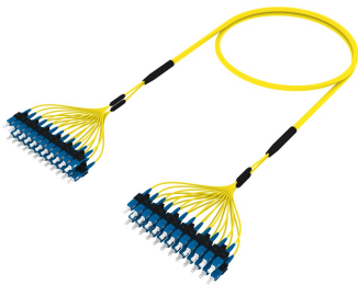
Fiber Optic Patch Cord, OS2, SC/UPC-SC/UPC, 24F RBR, 2.0 mm subunits, 56 m, yellow, 39"/60" breakouts
