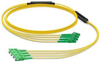
Fiber Optic Patch Cord, Multi-fiber, Singlemode, 4 fibers, LC/APC to SC /APC, yellow, 12 m
