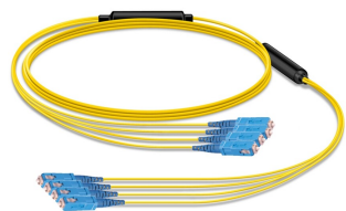
Fiber Optic Patch Cord, OS2, SC/UPC-SC/UPC, 4-fiber RBR, 2.0 mm subunits, 26 m, yellow, 25" breakouts
