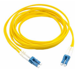
Fiber Optic Patch Cord, OS2, LC/UPC-LC/UPC, 2-fiber RBR, 2.0 mm subunits, 8 m, yellow, 39" breakouts
