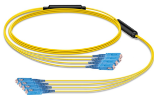
Fiber Optic Patch Cord, OS2, SC/UPC-SC/UPC, 4-fiber RBR, 2.0 mm subunits, 12 m, yellow, 39"/25" breakouts
