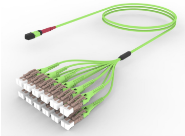
Ultra Low Loss OM5 MPO24 Unpinned to LC/UPC Uniboot 24-Fiber Low Smoke Zero Halogen/Riser Array Cord
