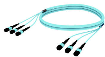
OM4 MPO12 (Pinned) to MPO12 (Unpinned), Fiber Trunk Cable Assembly, 36-Fiber, Method A, Plenum
