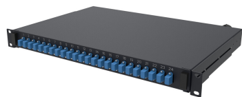
Fiber Optic Panel, 1U, 19 in, fully loaded with 24 blue LC/UPC Singlemode duplex adapters, black
