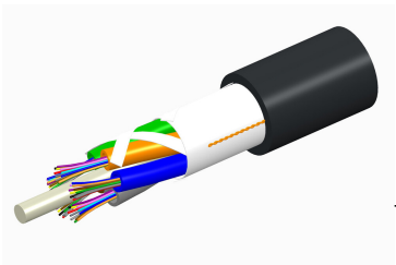
Fiber OSP cable, LazrSPEED® Single Jacket All-Dielectric, 144 fiber, Gel-Free, Stranded Loose Tube, Multimode OM4, Feet jacket marking, Black jacket color
